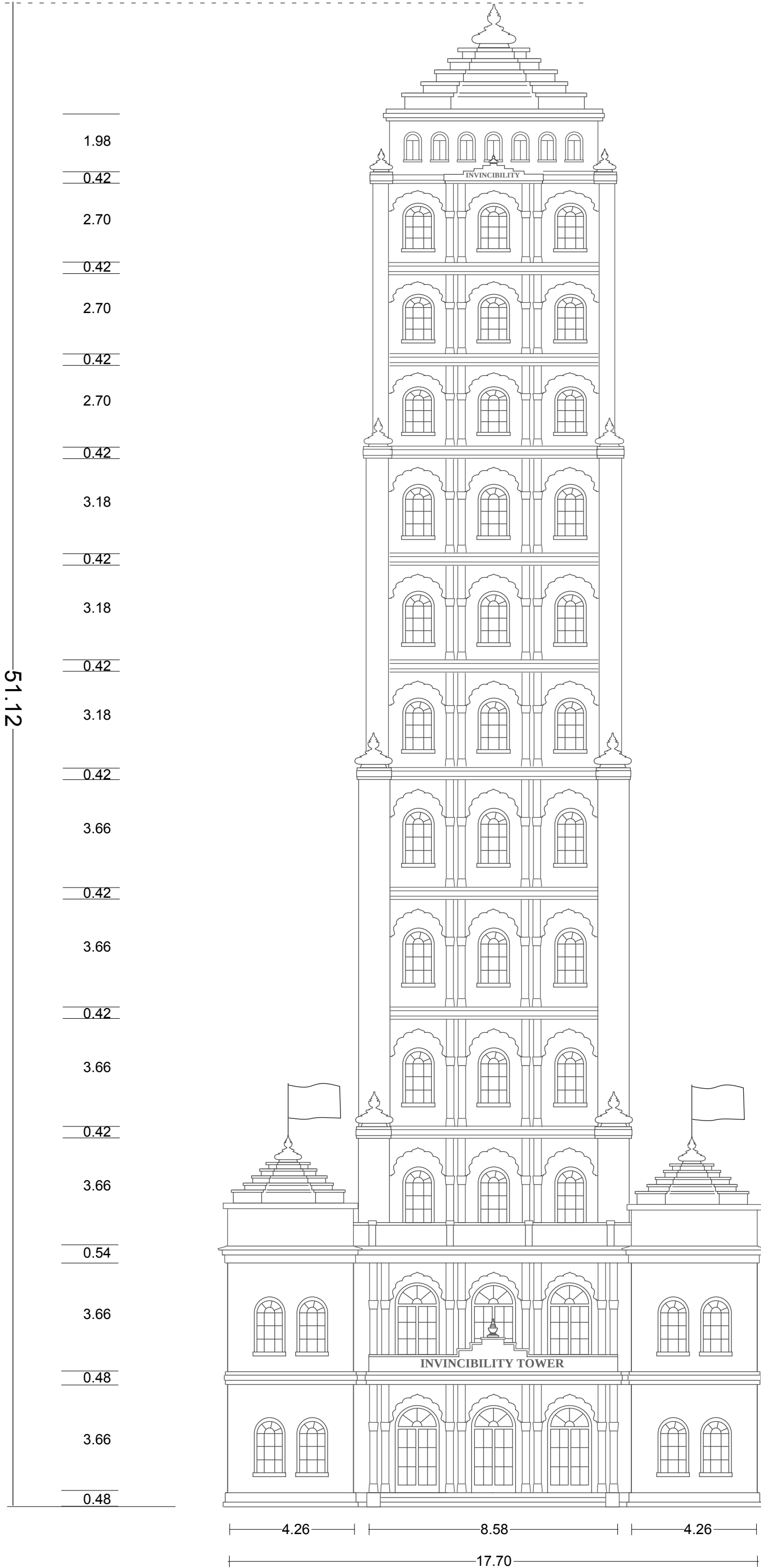
EAST ELEVATION
