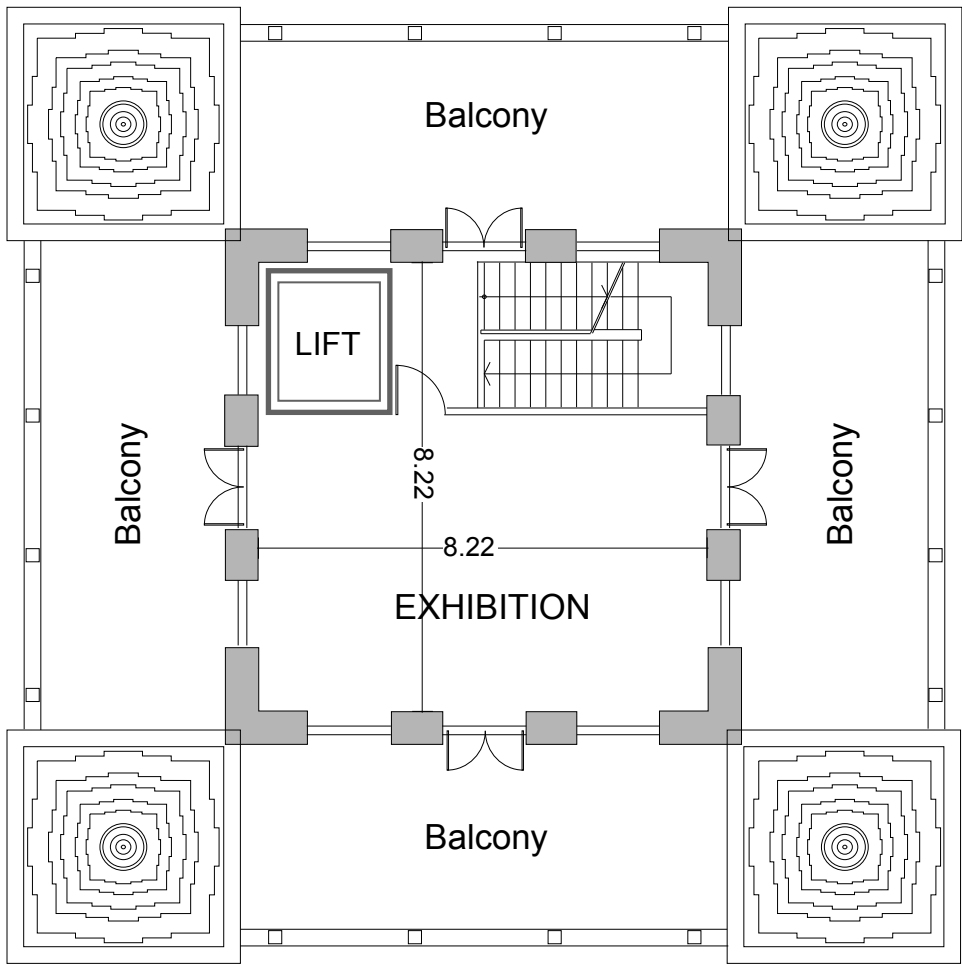
THIRD FLOOR
