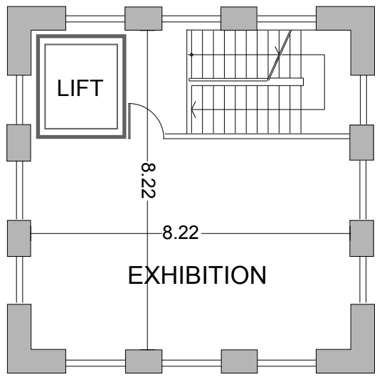
FLOORS 4-12
